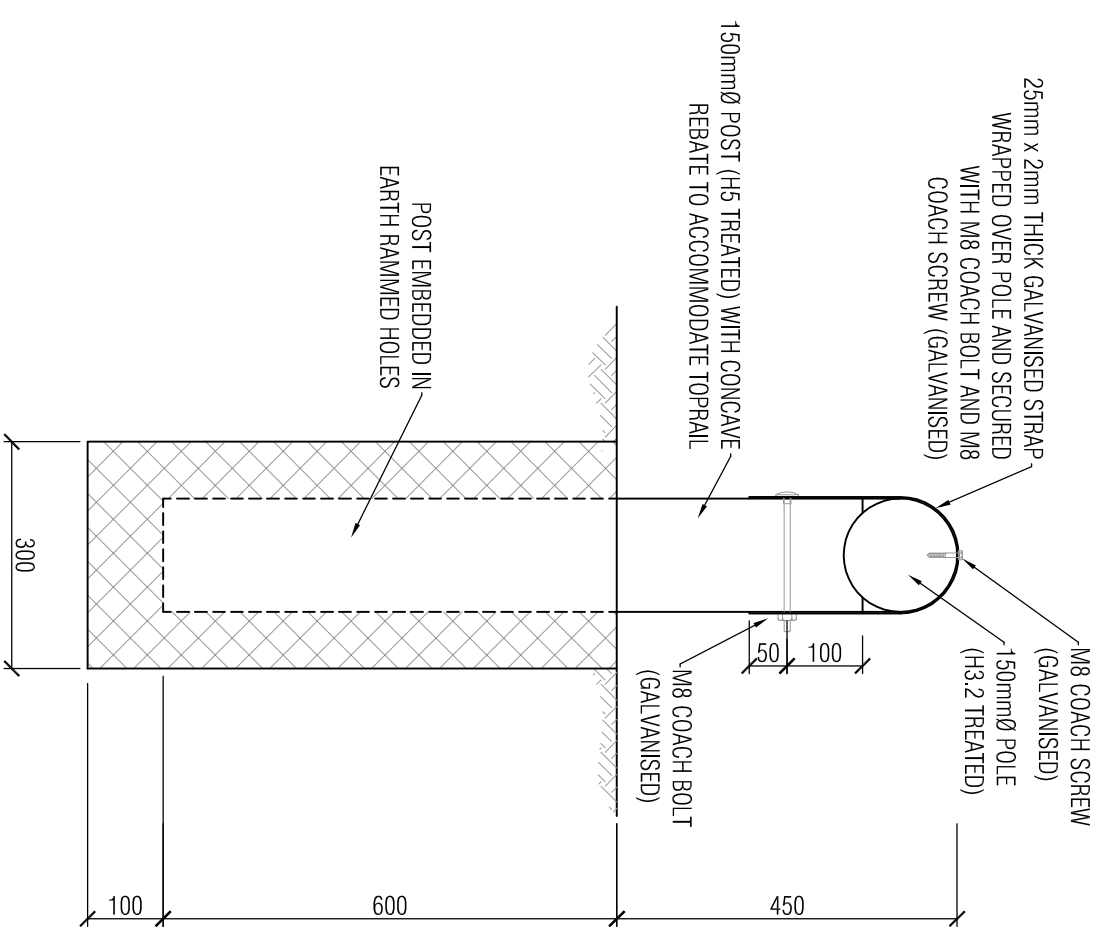
A POST AND TOPRAIL BARRIER - SECTION A SHT - 1:10
